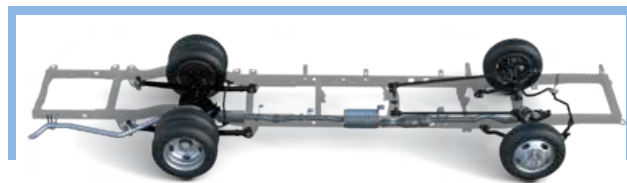
Rear suspension
